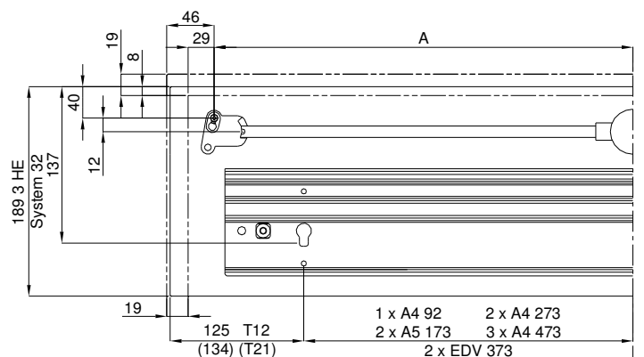
Ausziehbare Blende System 32 / Extending cover System 32
